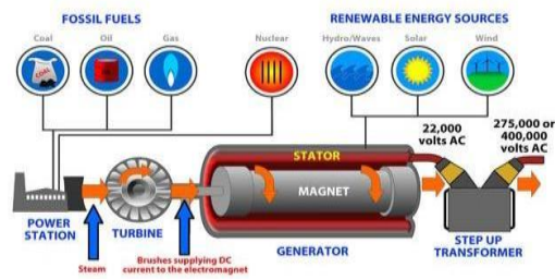
Fig.Usage of different energies for the production of electricity.
