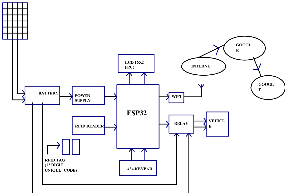
Figure 1: Block Diagram
